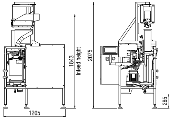
PEB41G for carrots Shaking collecting pan for alignment of carrots
